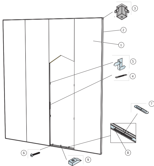
© Ecophon Installation diagram (M594C4) for Ecophon Akusto™ Wall C Akutex HS vertical installation with Connect Thinline Profile and distance.
