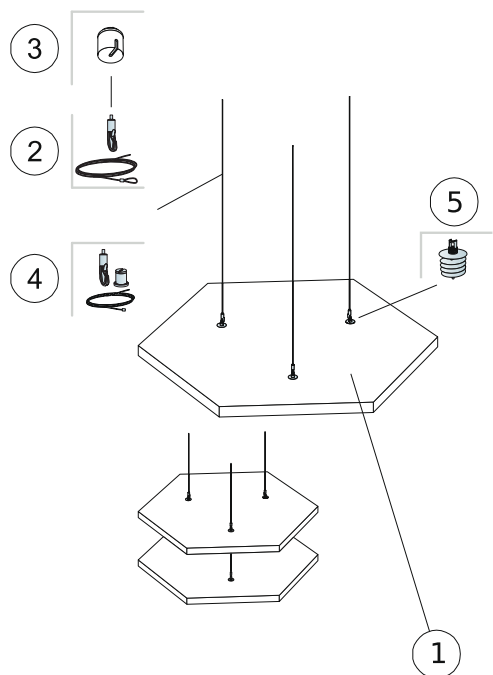
Installation diagram (M426) for Ecophon Solo Hexagon
