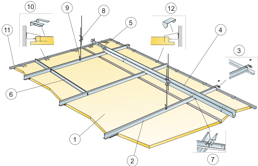
©Saint-Gobain Ecophon AB Installation diagram (M581) for Ecophon Focus Ds 600x600, 1200x600 mm and Ecophon Focus Ds XL. Suspended installation
